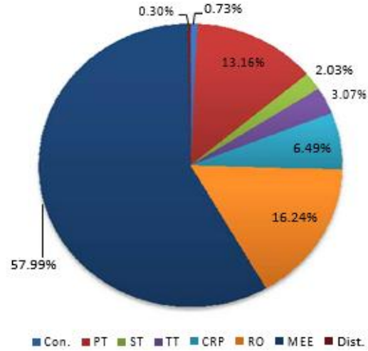
Figure 5.37: Typical Distribution of Total Opex of 64 MLD CETP Facility with MEE
