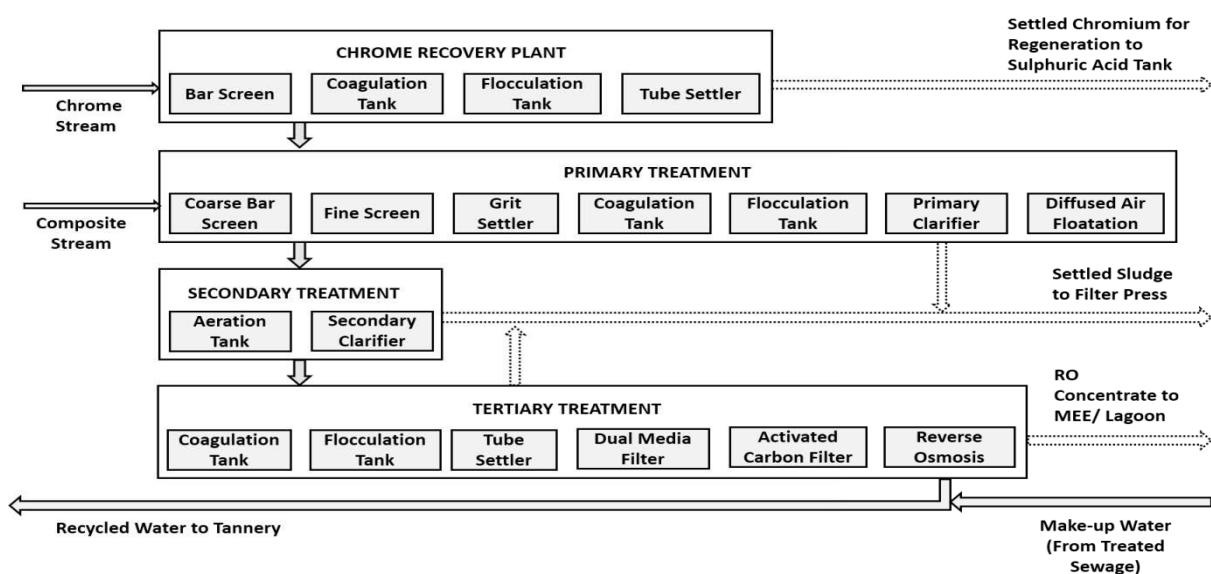
Figure 4.01: Schematic Flow Sheet for Treatment Facility of Tannery Effluent
