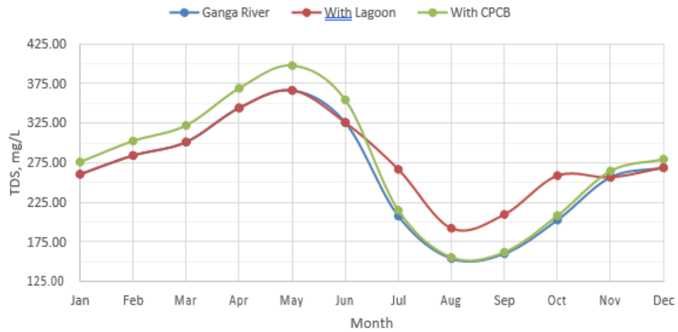
Figure 5.14: Monthly Average Concentrations in River Ganga, Post Discharge from Lagoon and Post Discharge as per CPCB Discharge Standards of Total Dissolved Solids in mg/L at Kanpur
