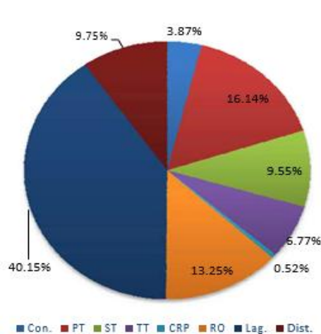
Figure 5.38: Typical Distribution of Total Capex of 64 MLD CETP Facility with Lagoon
