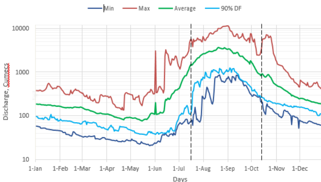
Figure 5.13: Representation of Hydrograph generated based on Daily Discharge Measurements by CWC during the period 1980-2009 at Bithoor Observation Station. The region between the dashed lines represent the period (15 July to 15 October) in which the concentrate will be discharged into the Ganga River.
