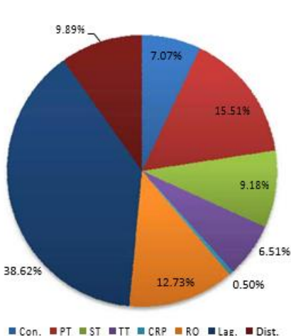
Figure 5.34: Typical Distribution of Total Capex of 32 MLD CETP Facility with Lagoon
