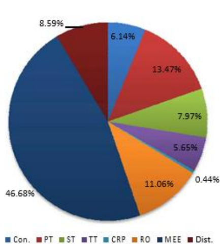
Figure 5.32: Typical Distribution of Total Capex of 32 MLD CETP Facility with MEE
