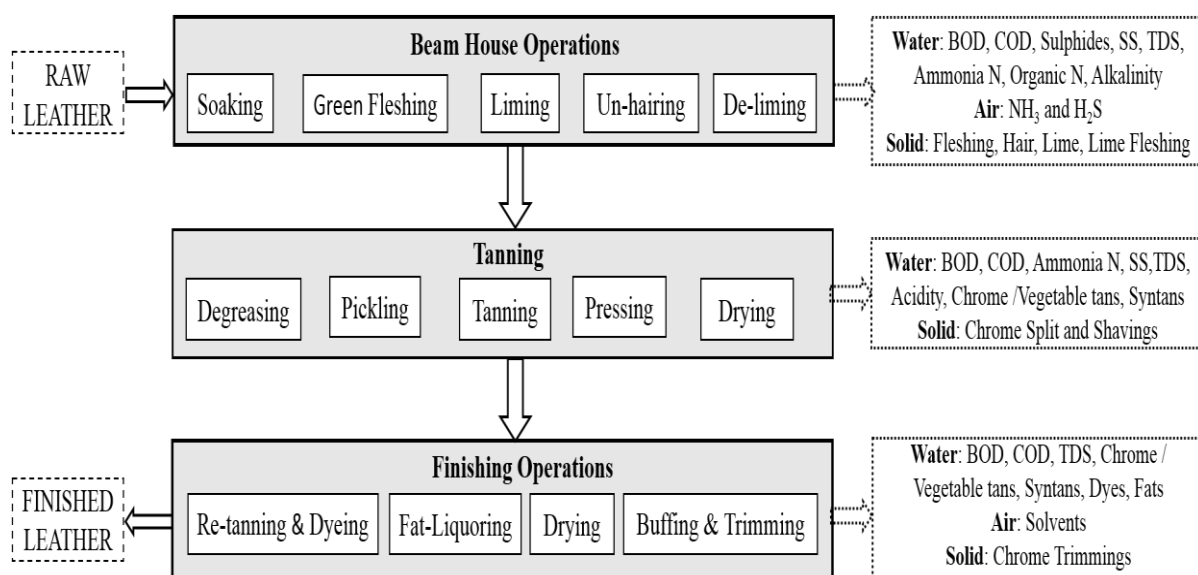
Figure 1.01: A typical process flow sheet in an integrated leather tanning industry with types of pollutants generated in leather processing
