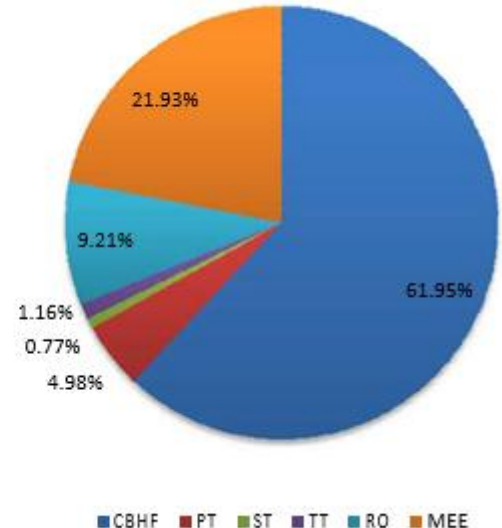
Figure 5.41: Typical Distribution of Total Opex of 12.8 MLD and 25.6 MLD CBHF Facility with MEE
