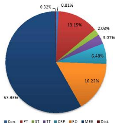
Figure 5.33: Typical Distribution of Total Opex of 32 MLD CETP Facility with MEE
