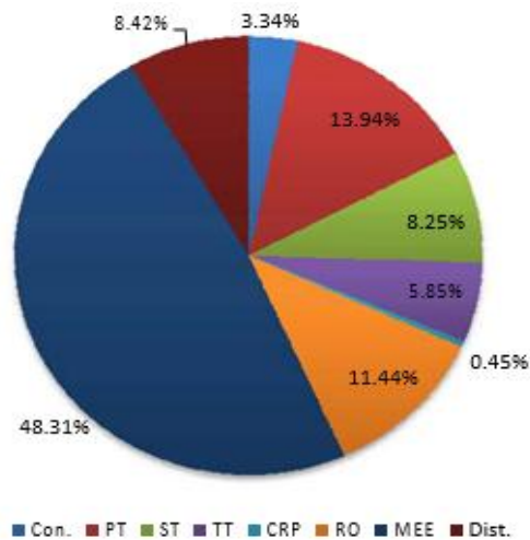
Figure 5.36: Typical Distribution of Total Capex of 64 MLD CETP Facility with MEE
