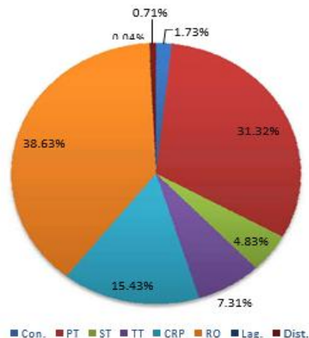
Figure 5.39: Typical Distribution of Total Opex of 64 MLD CETP Facility with Lagoon
