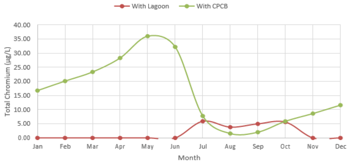
Figure 5.16: Monthly Average Concentrations in River Ganga, Post Discharge from Lagoon and Post Discharge as per CPCB Discharge Standards of Total Chromium in µg/L at Kanpur
