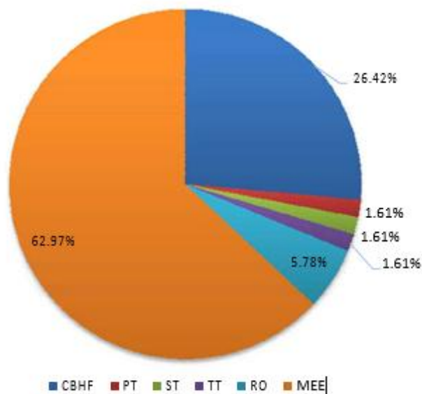
Figure 5.57: Typical Distribution of Total Energy Footprint of 25.6 MLD CBHF Facility with MEE
